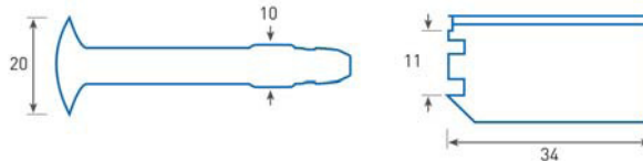
All Dimensions in mm
